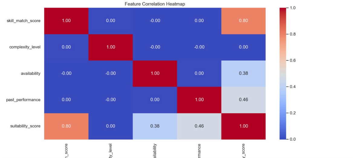
Figure 3.2: The feature correlation heatmap
