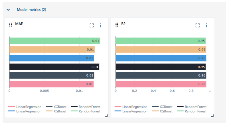
Figure 5.4: Model metrics graph from MLflow
